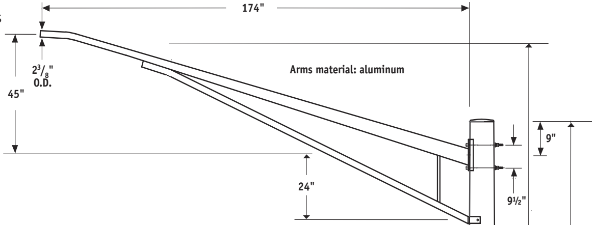
Truss Arm Dimensions
